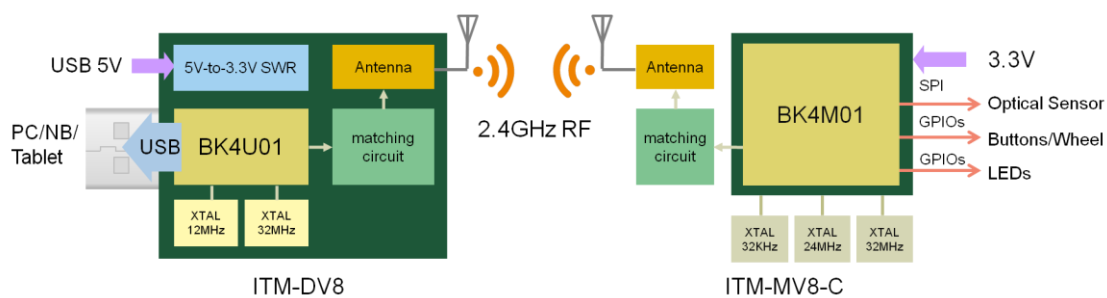
Block diagram of ITM-MV8-C / ITM-DV8
