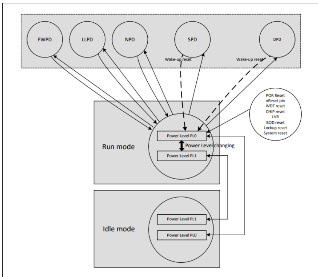
Figure 4.2-8 ITM-MV8-C Power Distribution Diagram
