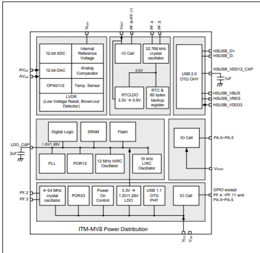
Figure 4.2-6 ITM-MV8-C Power Distribution Diagram
